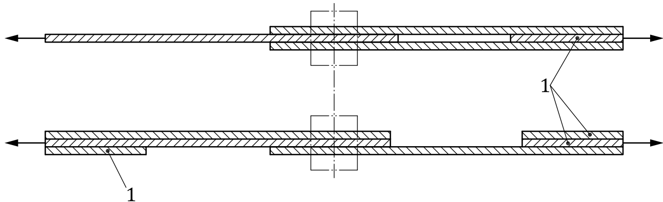
Key 1 shim plates
